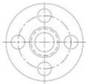
SS316 FLANGE - ANSI 150 - RF SLIP ON
